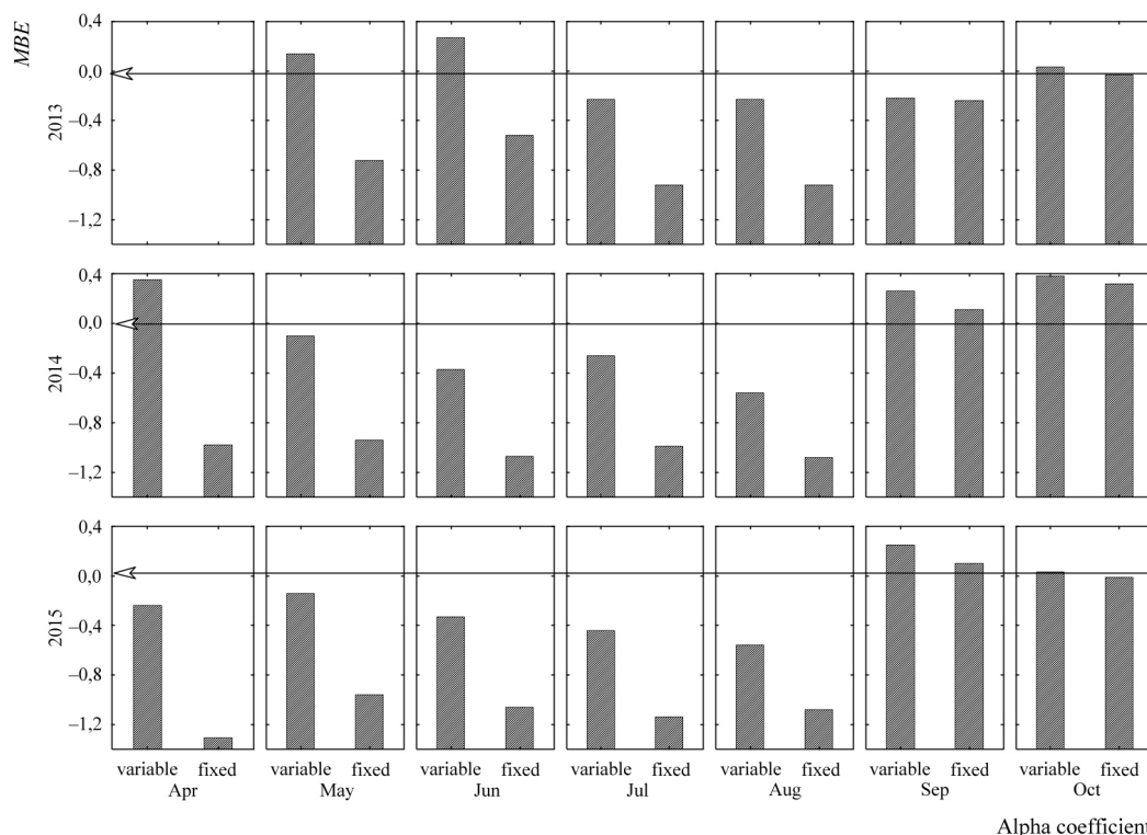
Fig. 5. Mean bias error ( MBE ) for ETo estimated by temperature, and fixed or variable coefficient \alpha in relation to the PMF56 reference model (Dąbrowie, 2013-2015)
