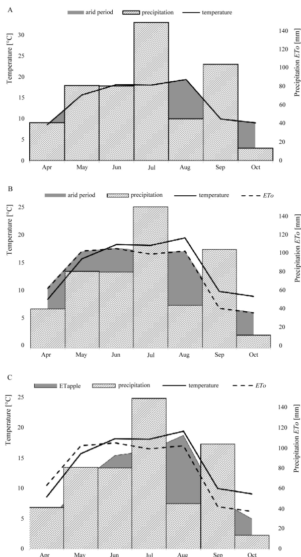
Fig. 7. Different versions of climate diagrams; A – traditional, B – new, C – new, including the value of the crop (apple) coefficient k (Słoje, 2013)
