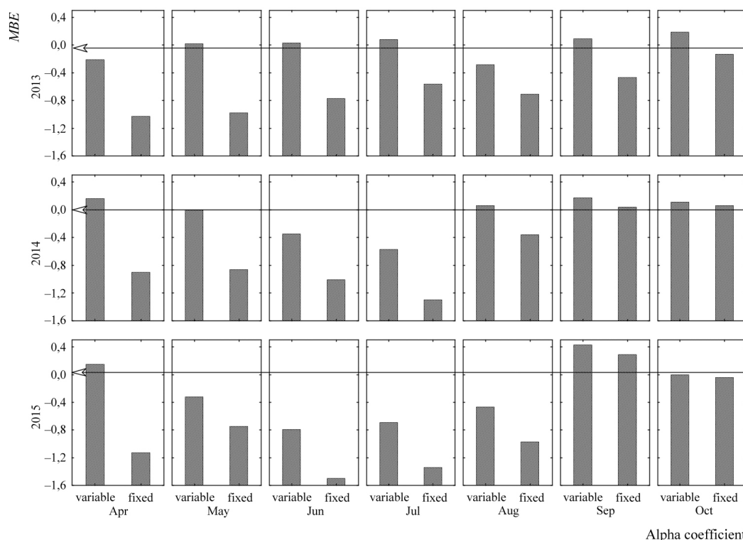
Fig. 4. Mean bias error ( MBE ) for ETo estimated by temperature, and fixed or variable coefficient \alpha in relation to the PMF56 reference model (Stoje, 2013-2015)
