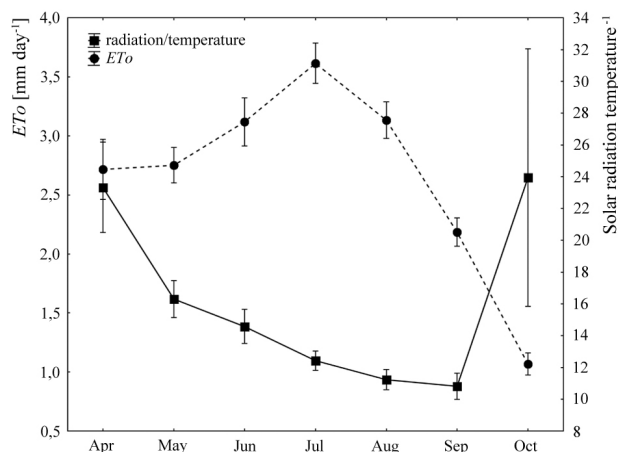
Fig. 2. Variations in ET_0 and the indicator of the level of radiation per unit temperature; mean values for all the stations and years of the study
