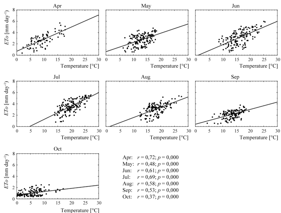
Fig. 3. The relationship between temperature and evapotranspiration in each month of the growing season; aggregate data for the stations and years of the study
